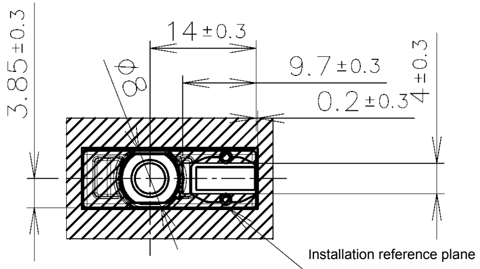
Figure 5: Optical Clear Area of Exit Window
