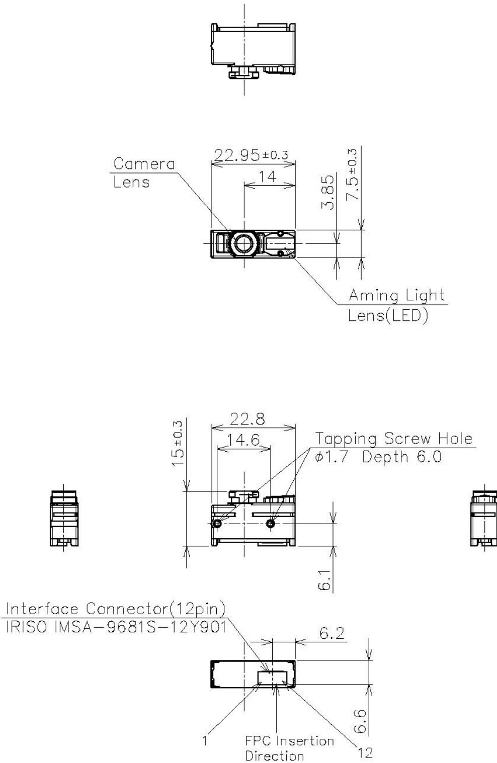
Figure 11: Mechanical Drawing
